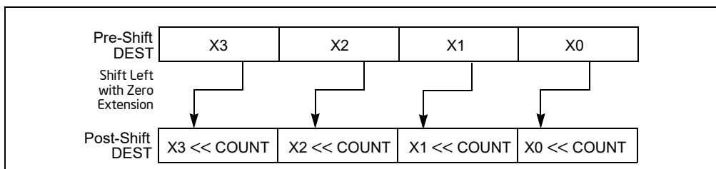
Figure 4-17. PSSLW, PSLLD, and PSLLQ Instruction Operation Using 64-bit Operand
