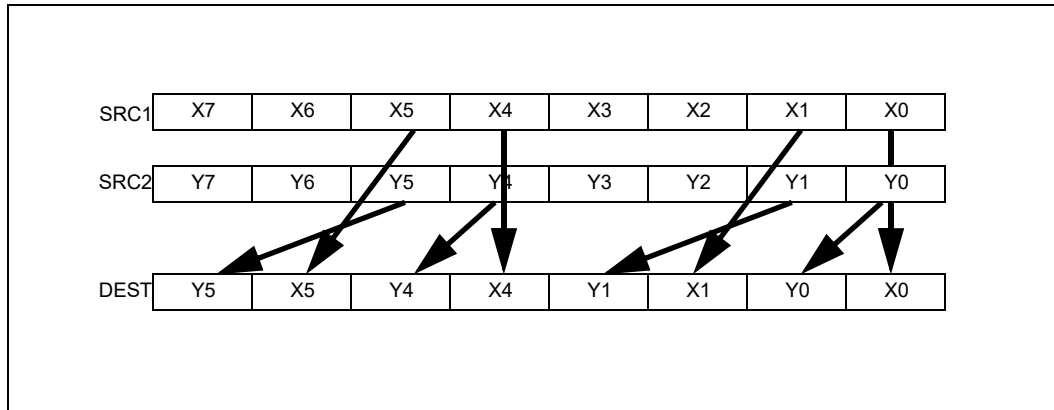
Figure 4-28. VUNPCKLPS Operation
