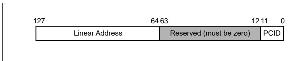
Figure 3-25. INVPCID Descriptor
