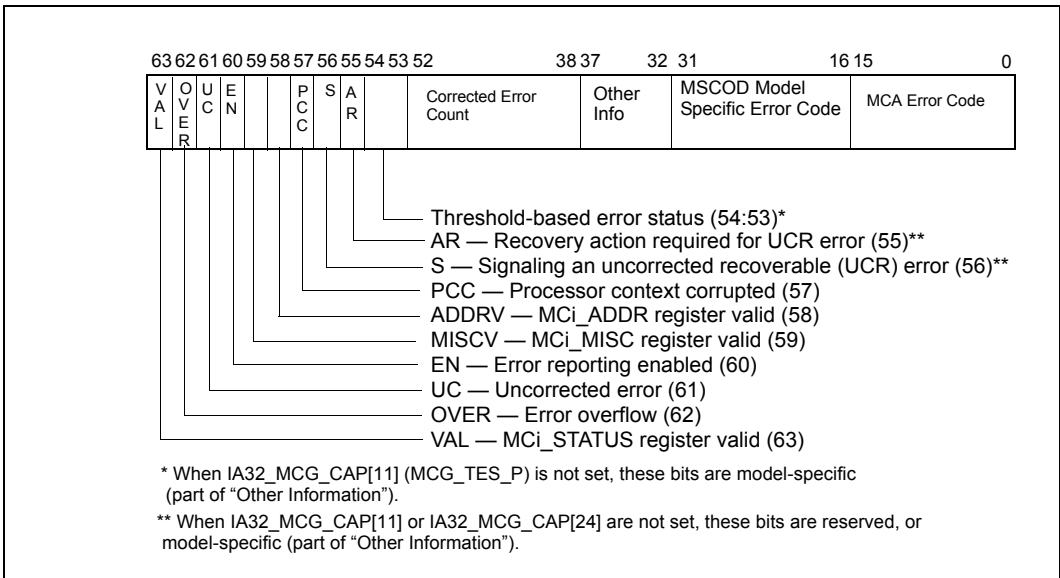
Figure 15-5. IA32_MCI_STATUS Register
