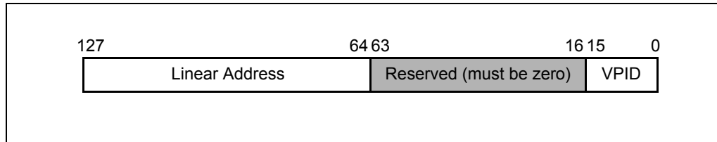
Figure 29-2. INVVPID Descriptor
