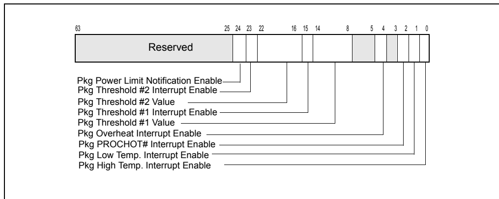
Figure 14-15. IA32_PACKAGE_THERM_INTERRUPT Register
