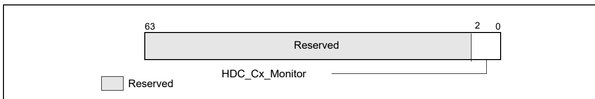
Figure 14-22. MSR_PKG_HDC_CONFIG MSR
