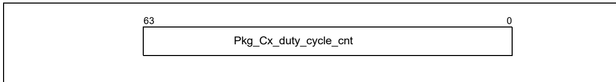
Figure 14-21. MSR_PKG_HDC_DEEP_RESIDENCY MSR
