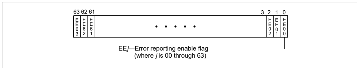
Figure 15-5. IA32_MCi_CTL Register
