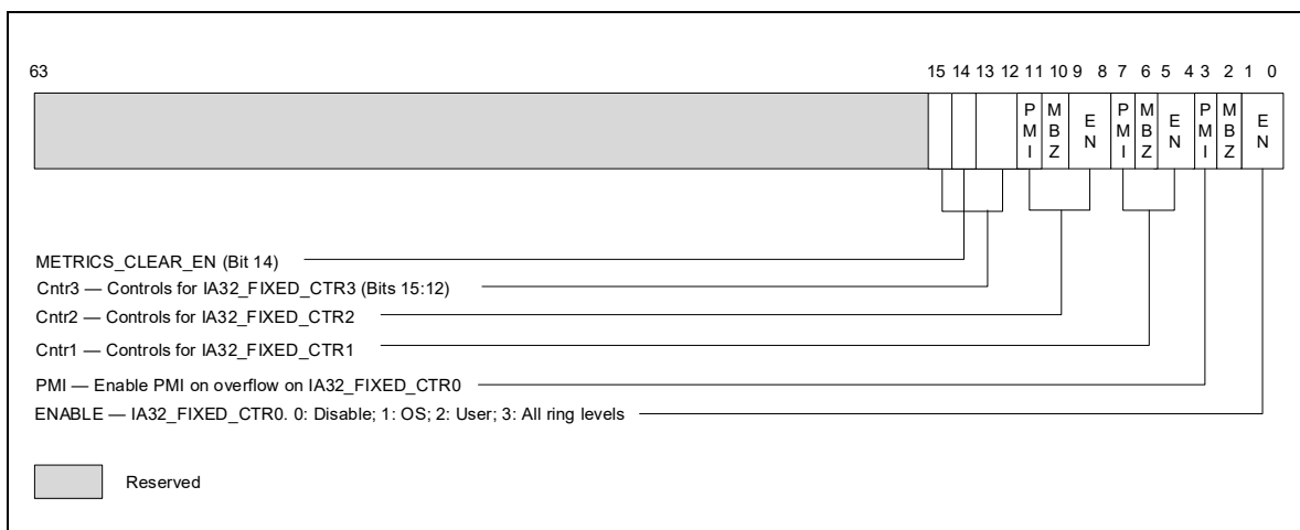
Figure 21-15. IA32_FIXED_CTR_CTRL MSR Supporting Architectural Performance Monitoring Version 6
