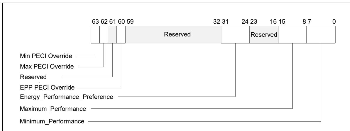
Figure 16-8. IA32_HWP_PECI_REQUEST_INFO MSR
