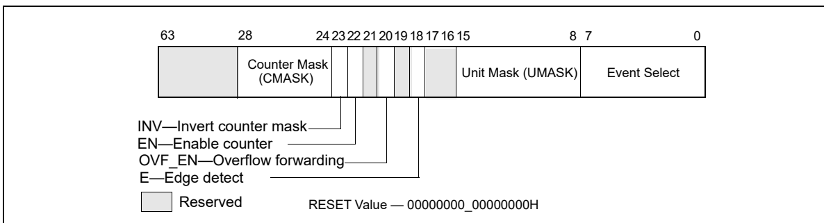
Figure 21-34. Layout of Uncore PERFECTSEL MSR for a C-Box Unit or the ARB Unit
