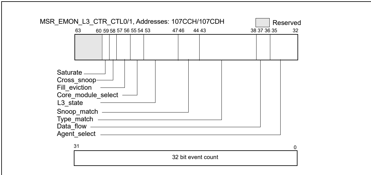
Figure 21-62. MSR_EMON_L3_CTL0/1, Addresses: 107CCH/107CDH
