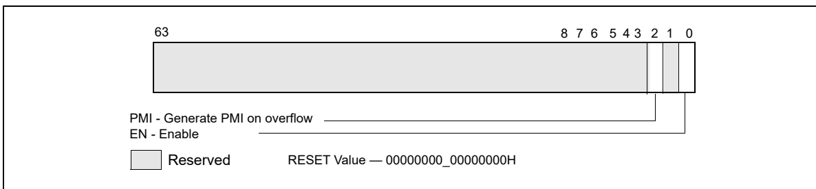
Figure 21-25. Layout of MSR_UNCORE_FIXED_CTR_CTRL MSR
