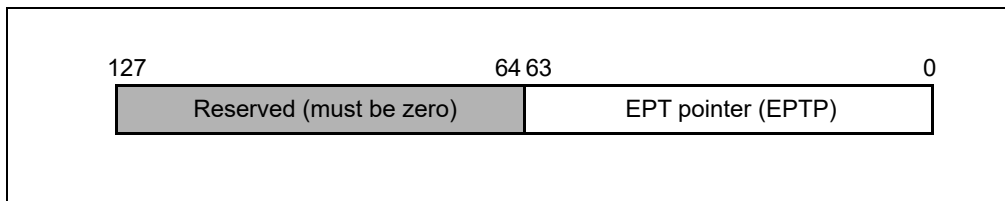
Figure 32-1. INVEPT Descriptor
