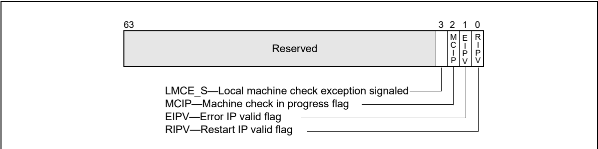
Figure 17-3. IA32_MCG_STATUS Register
