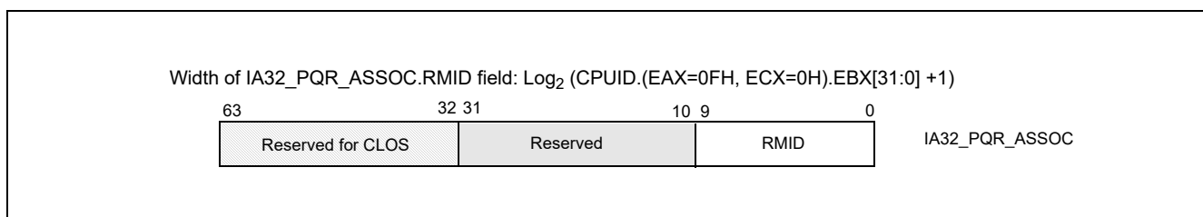
Figure 19-23. IA32_PQR_ASSOC MSR
