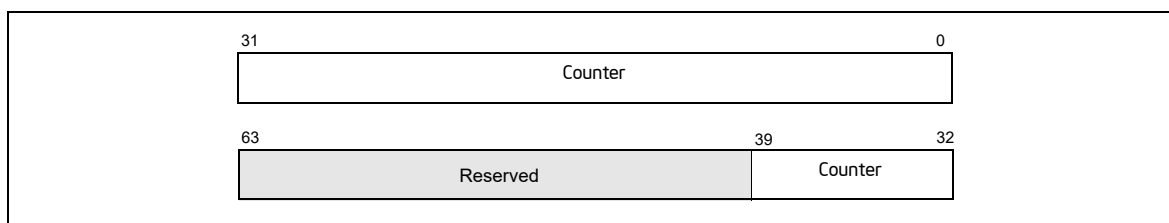
Figure 21-50. Performance Counter (Pentium 4 and Intel® Xeon® Processors)
