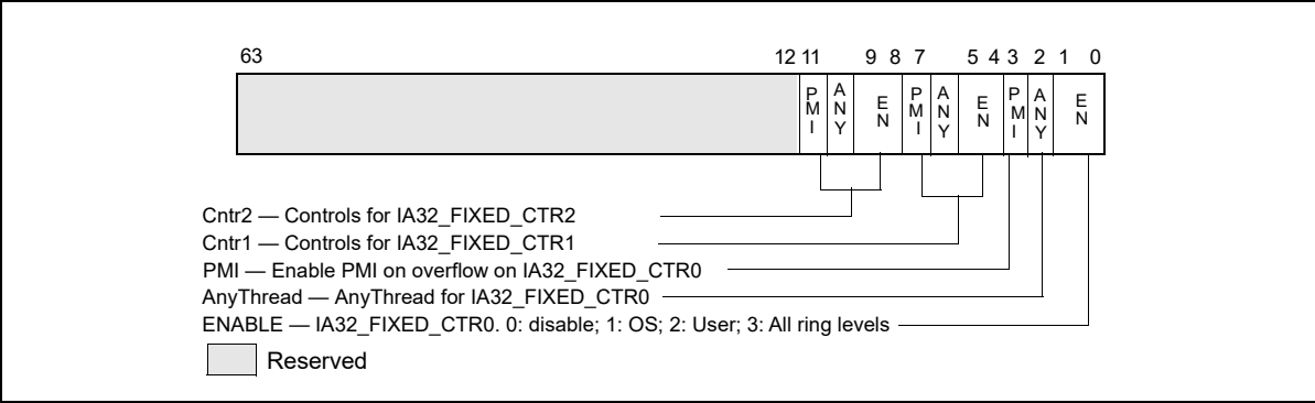
Figure 21-7. IA32_FIXED_CTR_CTRL MSR Supporting Architectural Performance Monitoring Version 3
