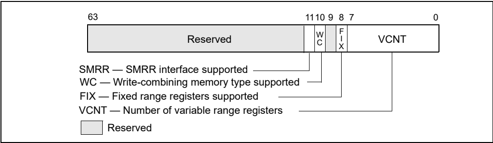
Figure 13-5. IA32_MTRRCAP Register
