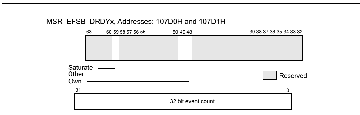
Figure 21-58. MSR_EFSB_DRDYx, Addresses: 107D0H and 107D1H
