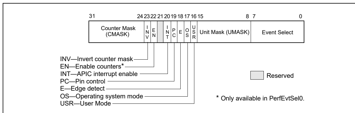
Figure 21-65. PerfEvtSel0 and PerfEvtSel1 MSRs
