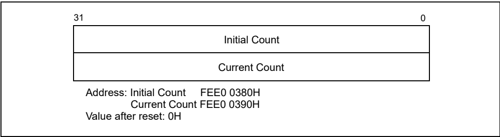
Figure 13-11. Initial Count and Current Count Registers
