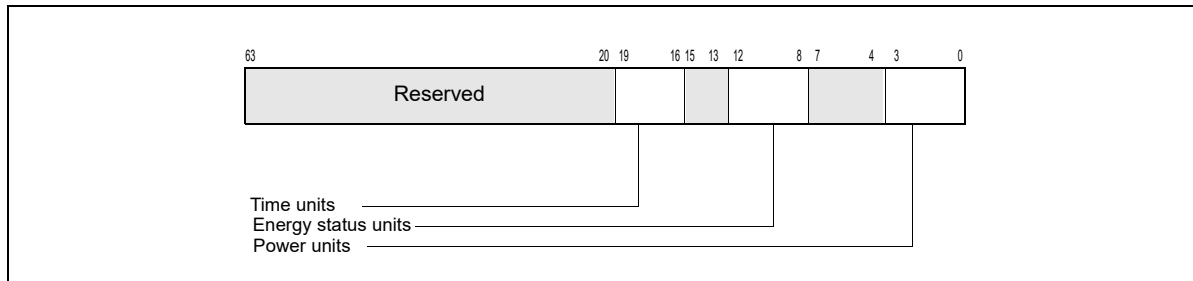
Figure 17-35. MSR_RAPL_POWER_UNIT Register
