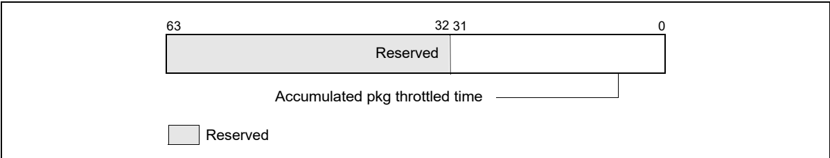
Figure 17-39. MSR_PKG_PERF_STATUS MSR
