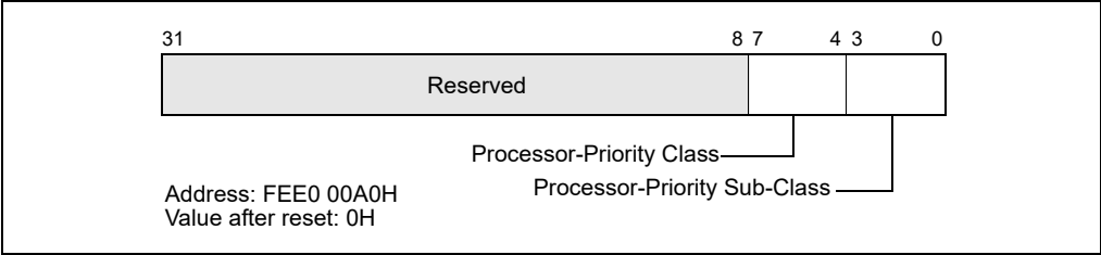
Figure 13-19. Processor-Priority Register (PPR)
