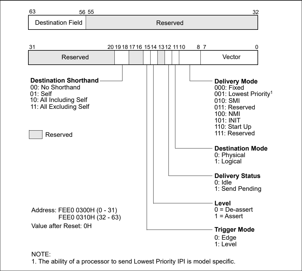
Figure 13-12. Interrupt Command Register (ICR)
