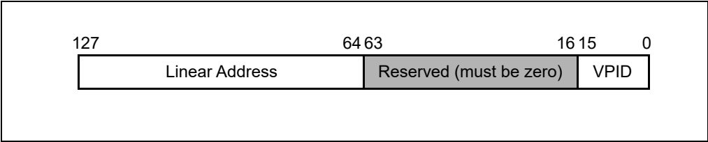
Figure 32-2. INVVPID Descriptor
