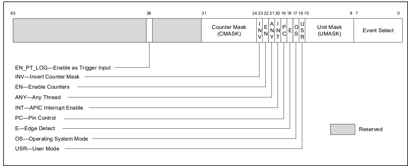
Figure 36-4. Layout of the IA32_PERFEVTSELx MSR
