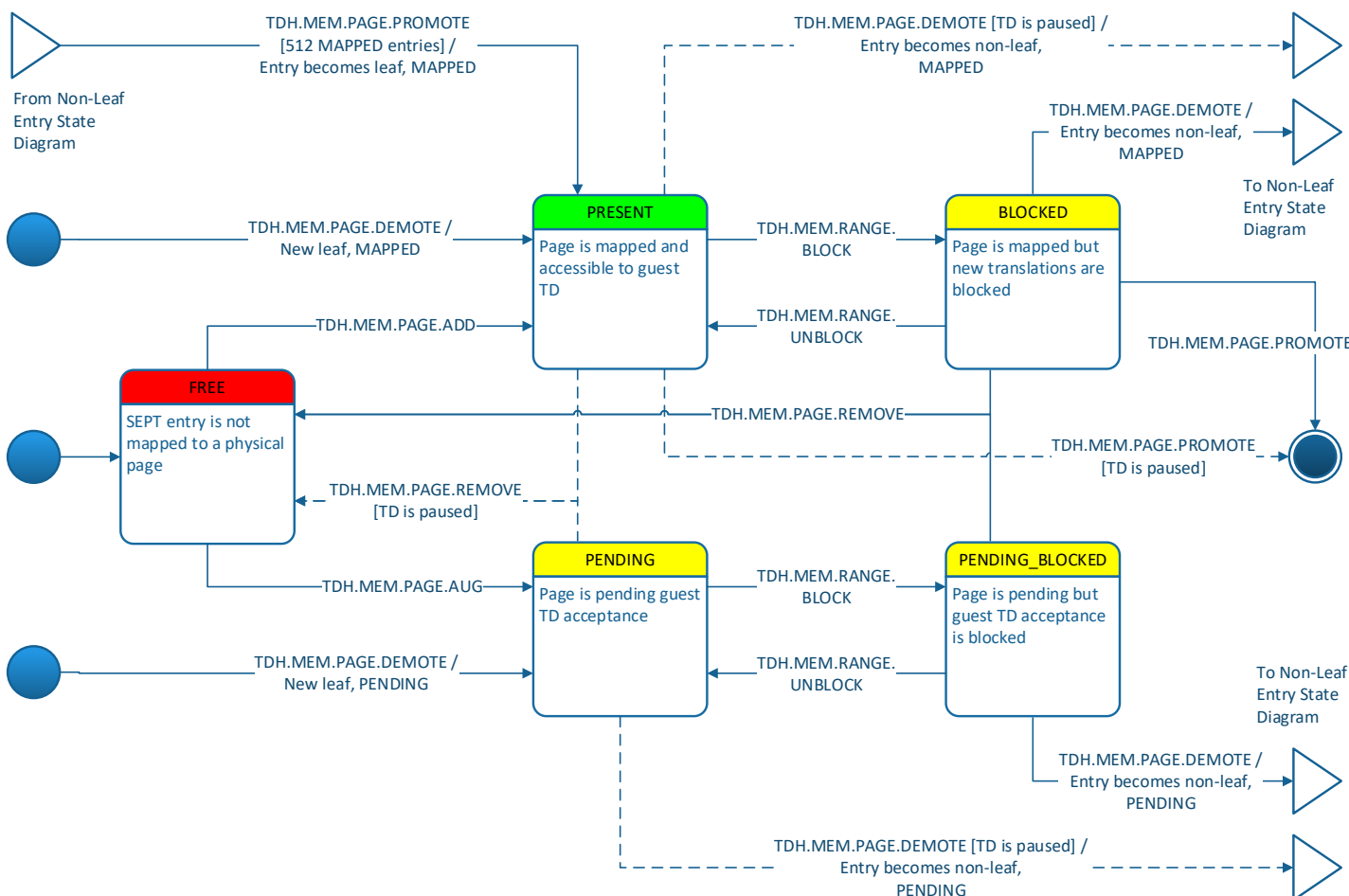
Figure 8.2: Secure EPT Leaf Entry Partial State Diagram
