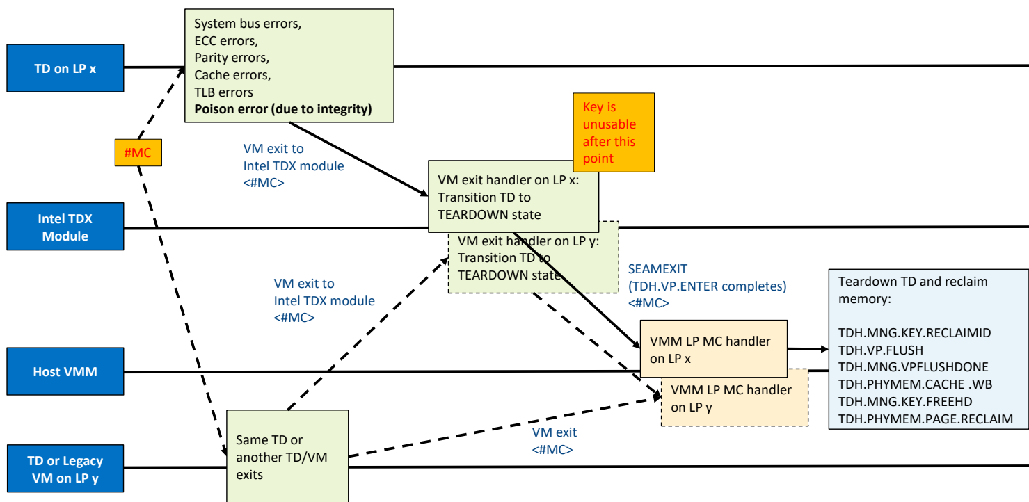
Figure 15.1: Example of Machine Check Handling and TD Memory Reclamation
