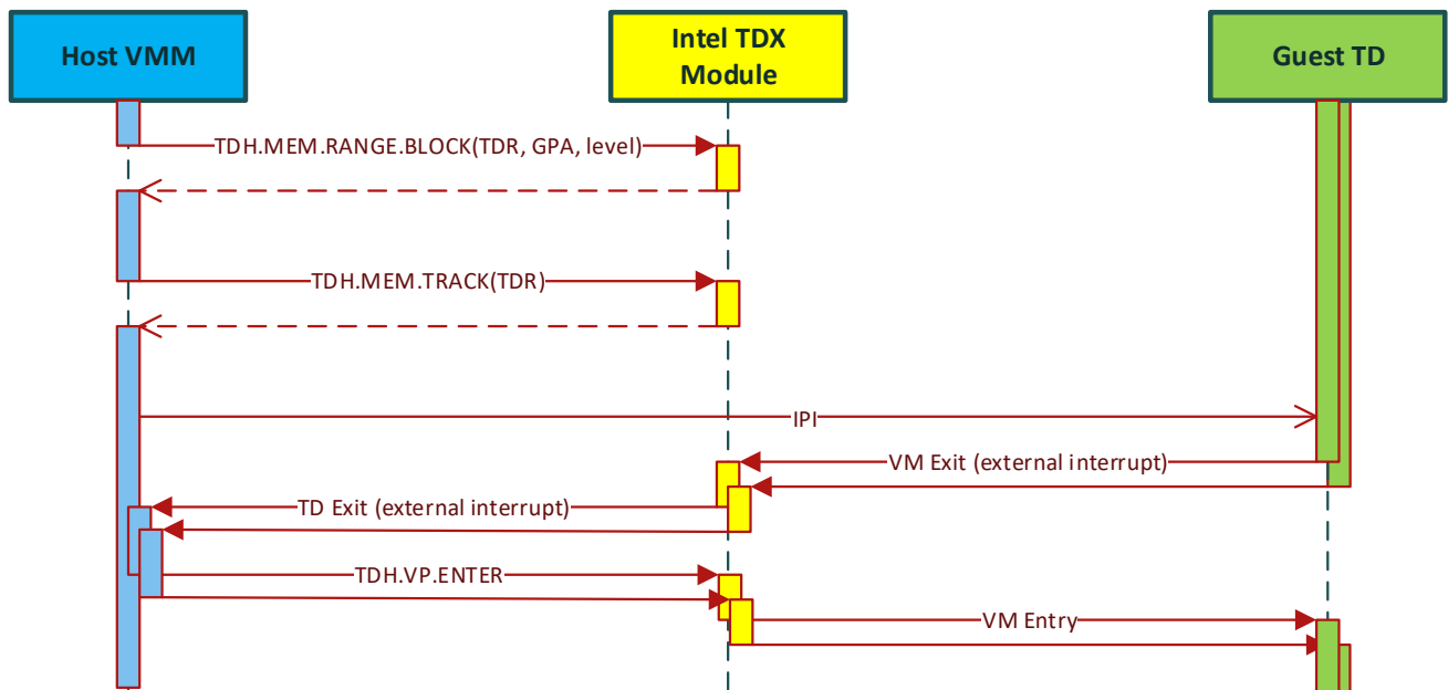
Figure 8.4: Typical TLB Tracking Sequence
