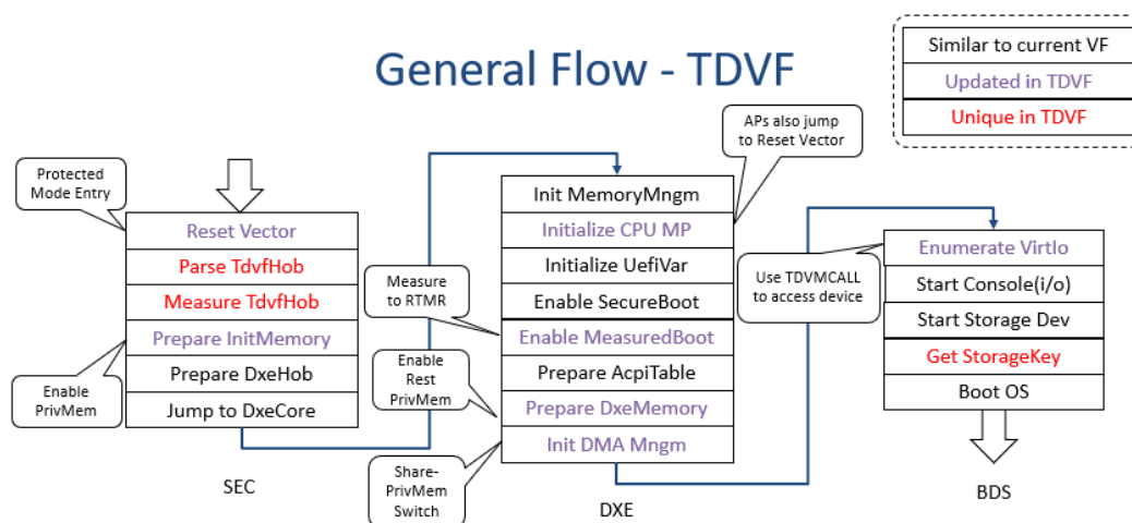
Figure 4-1: TDVF General Flow
