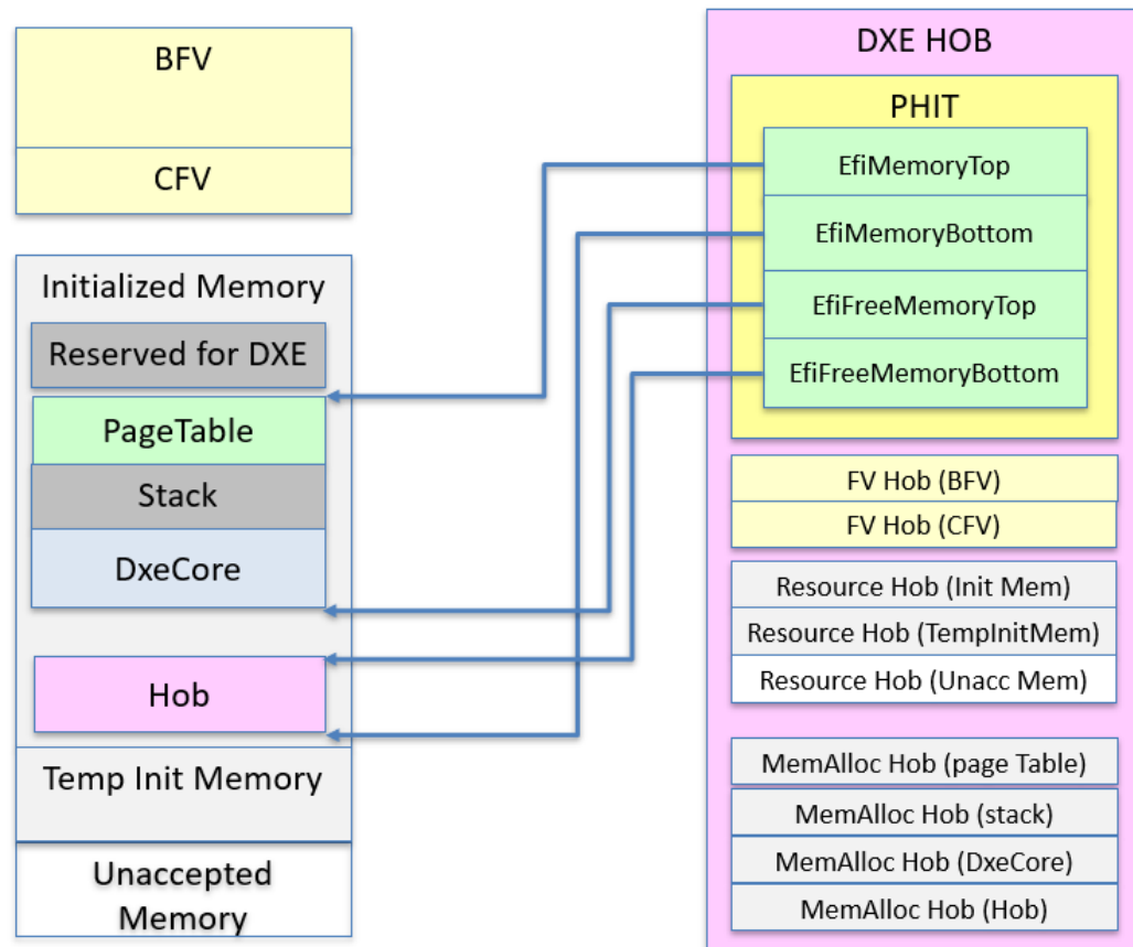
Figure 7-2: DXE HOB and Runtime Memory Layout
