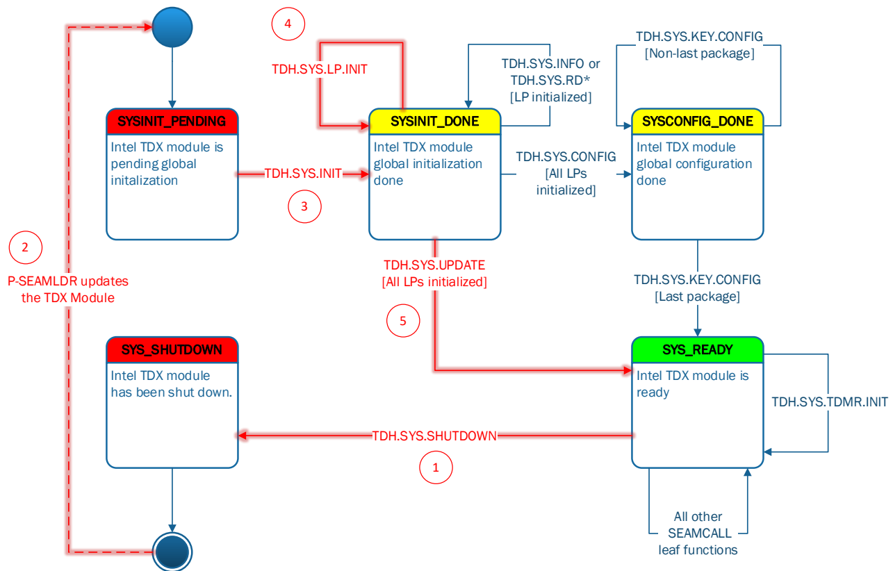
Figure 4.4: TDX Module Lifecycle State Machine – TD-Preserving Update
