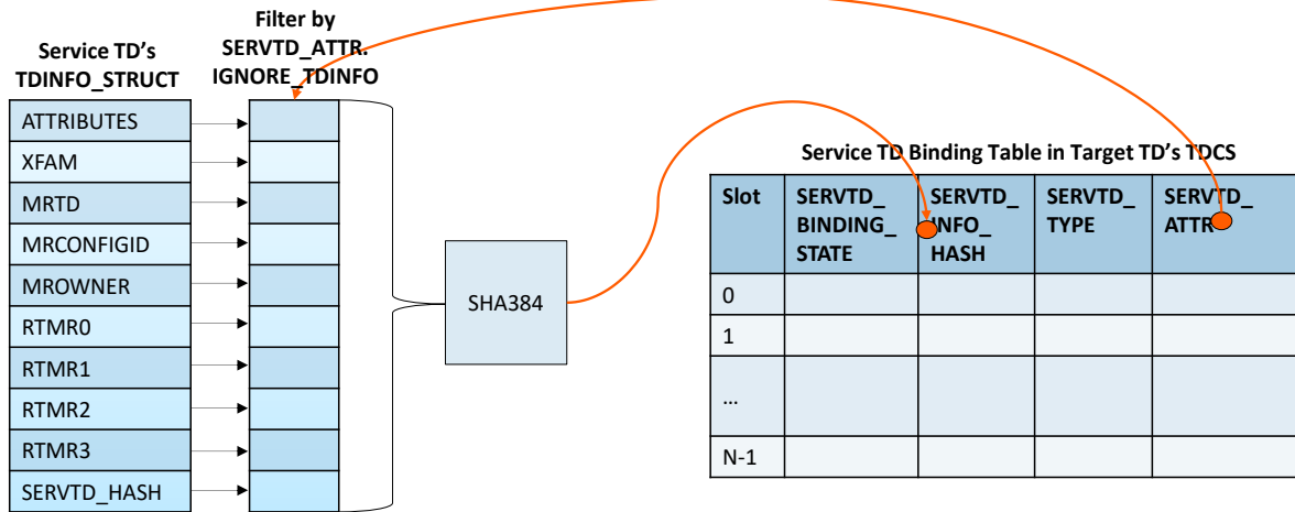
Figure 13.2: SERVTD_INFO_HASH Calculation
