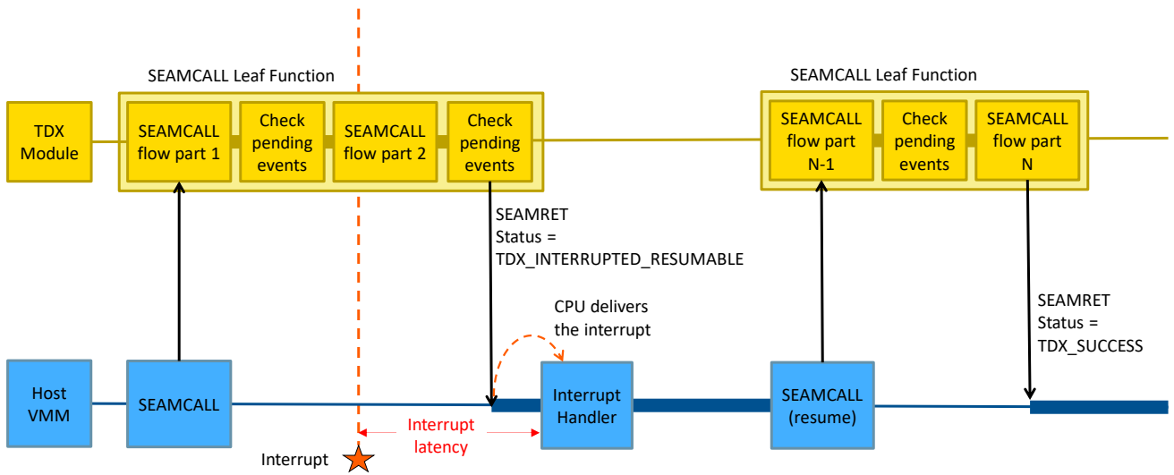
Figure 18.16: Typical Interruptible & Resumable SEAMCALL Leaf Function
