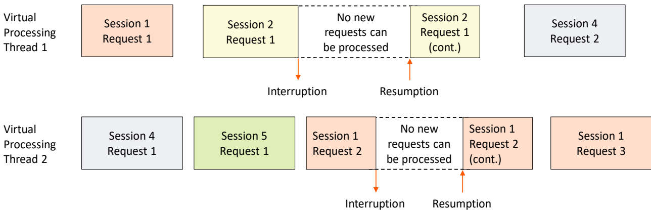
Figure 18.7: Request Interruption and Resumption as Part of Sessions
