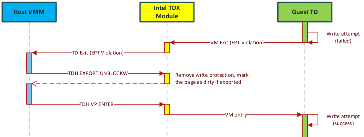
Figure 8.6: Typical Sequence for Unblocking a Page on Guest TD Write Attempt
