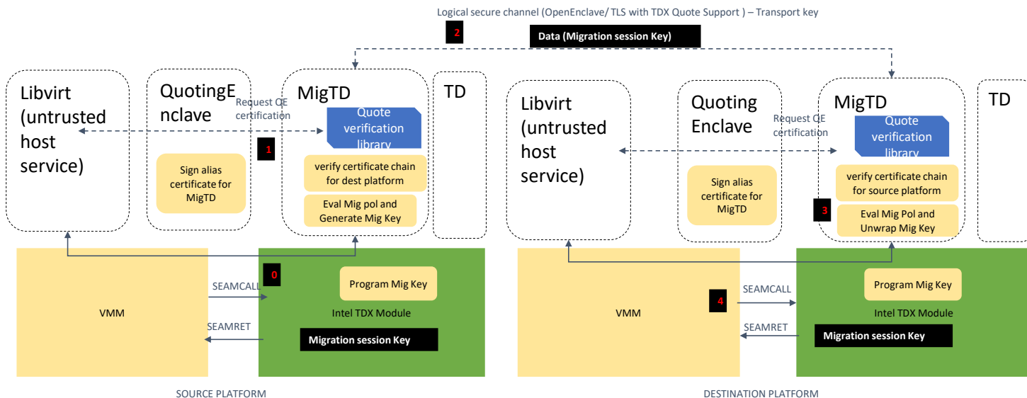
Figure 4.2: MigTD Transport Security Setup
