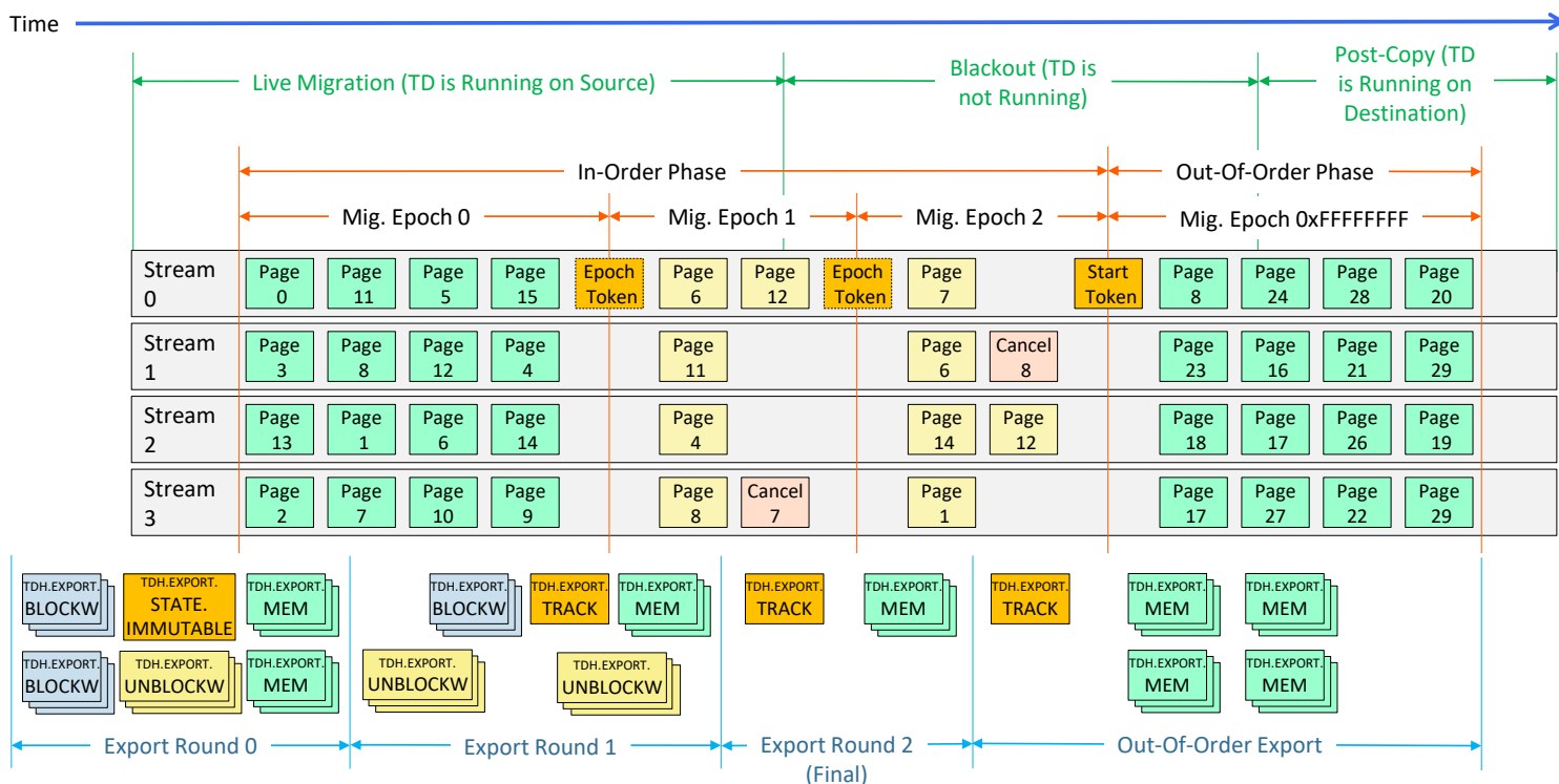
Figure 8.1: Migration Epochs
