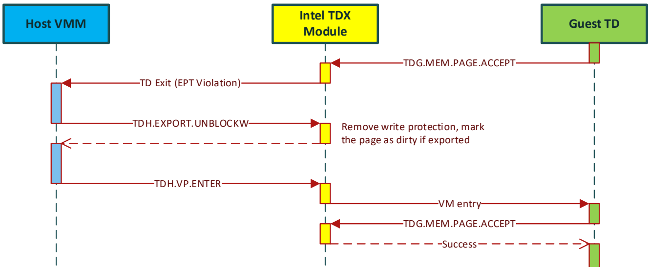
Figure 8.10: Typical Sequence for Unblocking a PENDING Page on TDG.MEM.PAGE.ACCEPT Attempt
