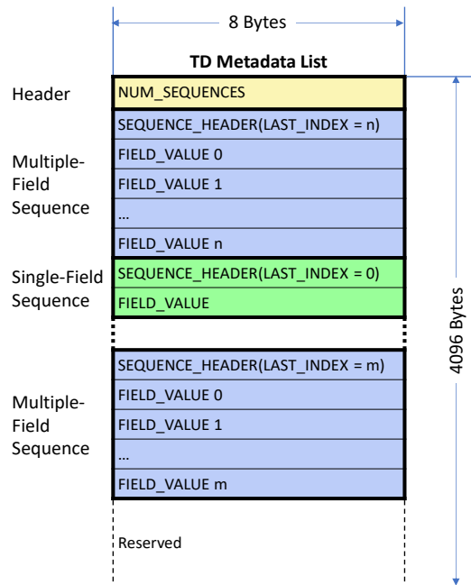
Figure 7.1: Non-Memory State Migration Page
