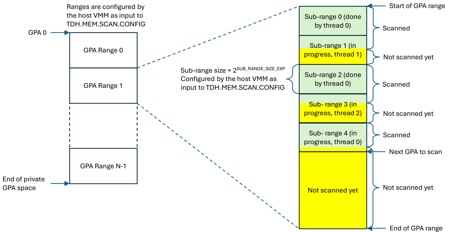
Figure 5.4: Concurrent Scan within a GPA Range
