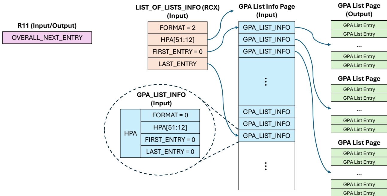
Figure 5.3: GPA List of Lists as Used by TDH.MEM.SCAN.COMP/RANGE
