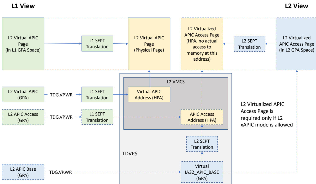
Figure 23.3: APIC Virtualization
