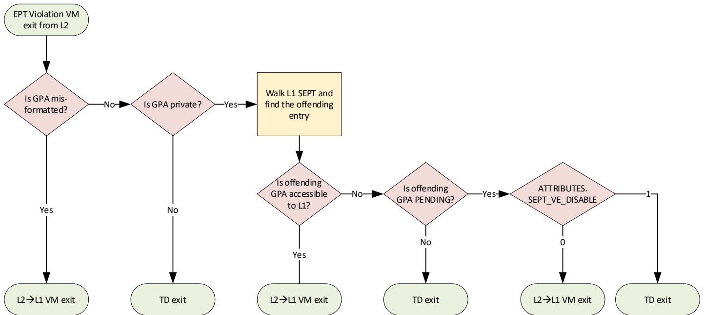
Figure 21.8: Handling EPT Violation VM Exit from L2
