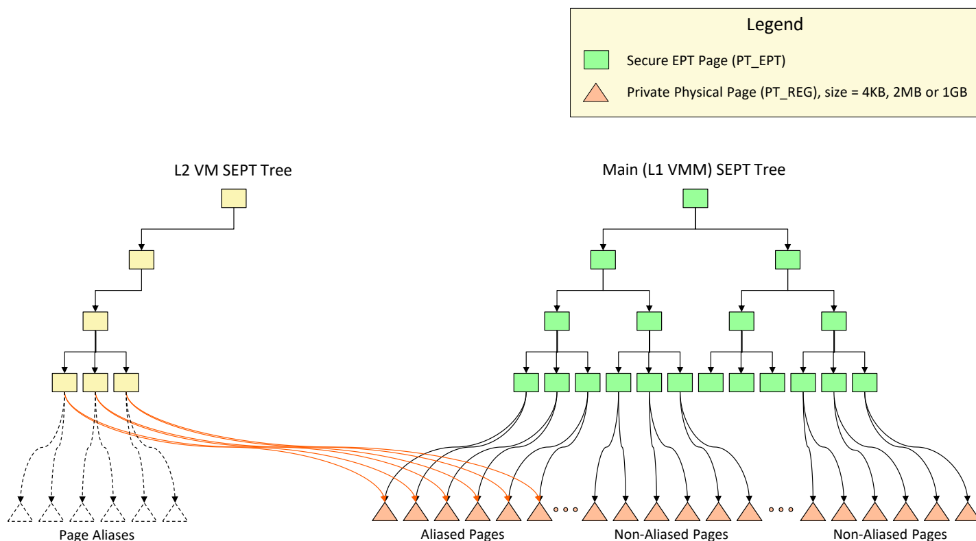
Figure 21.2: Page Aliasing
