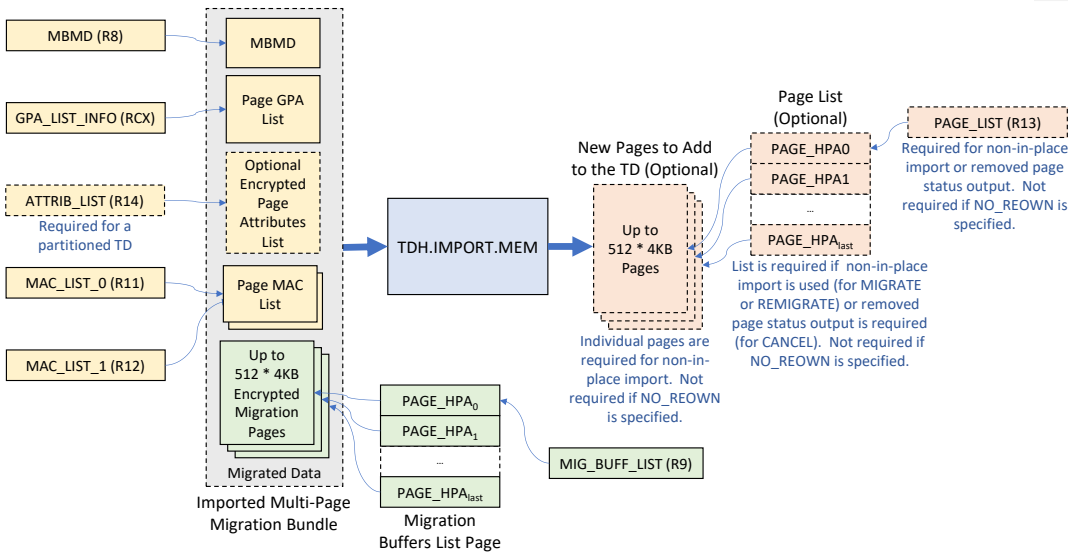
Figure 3.2: TDH.IMPORT.MEM Inputs and Outputs
