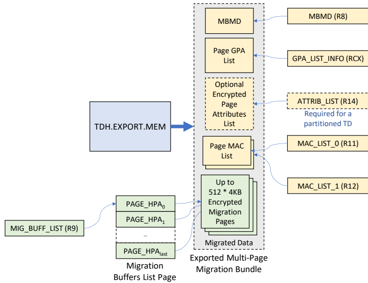
Figure 3.1: TDH.EXPORT.MEM Inputs and Outputs
