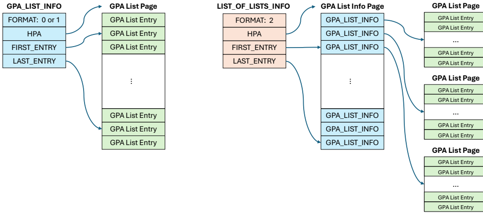
Figure 2.1: GPA List and List of Lists
