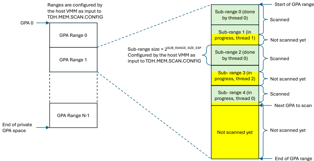
Figure 3.4: Concurrent Scan within a GPA Range
