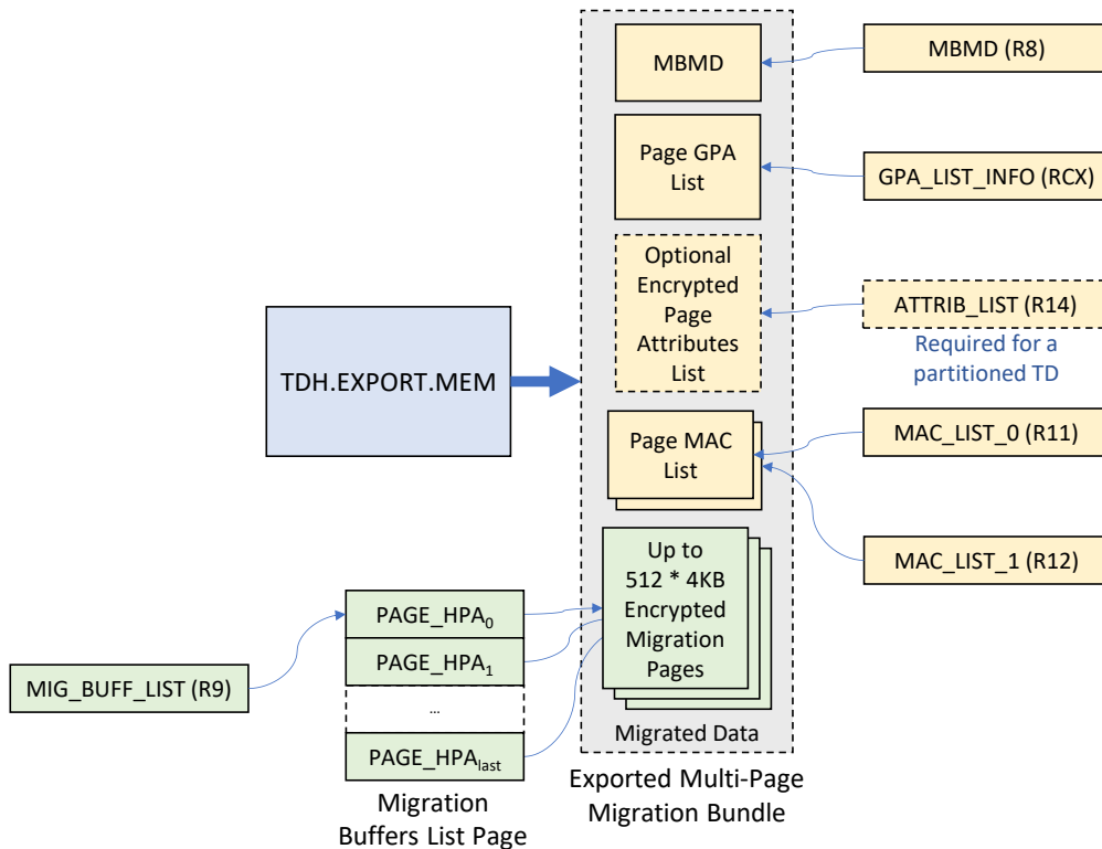
Figure 3.1: TDH.EXPORT.MEM Inputs and Outputs
