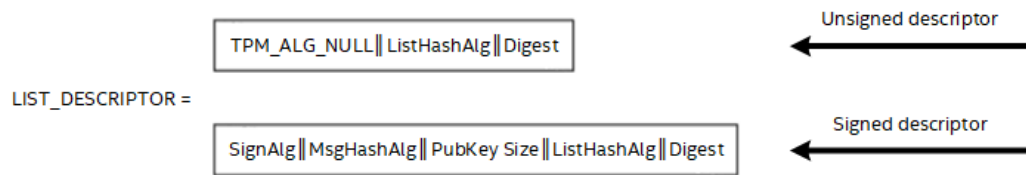
Figure 9: List Descriptor
