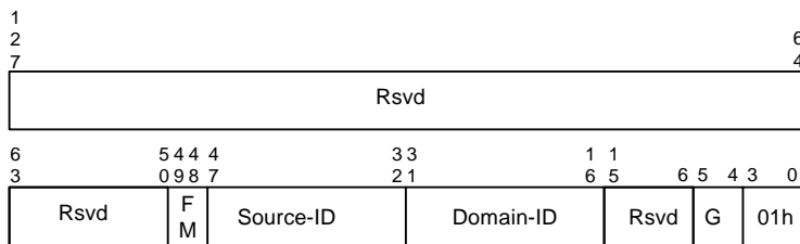
Figure 6-17. Context Cache Invalidate Descriptor
