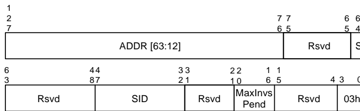
Figure 6-19. Device-IOTLB Invalidate Descriptor
