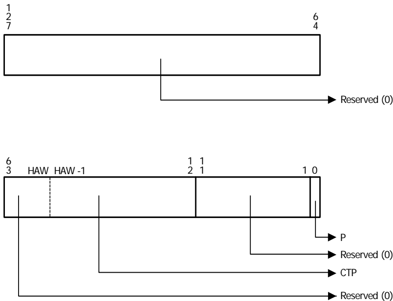
Figure 9-23. Root-Entry Format
