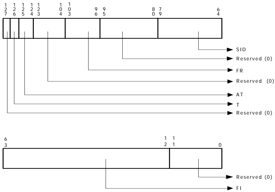
Figure 9-26. Fault-Record Format
