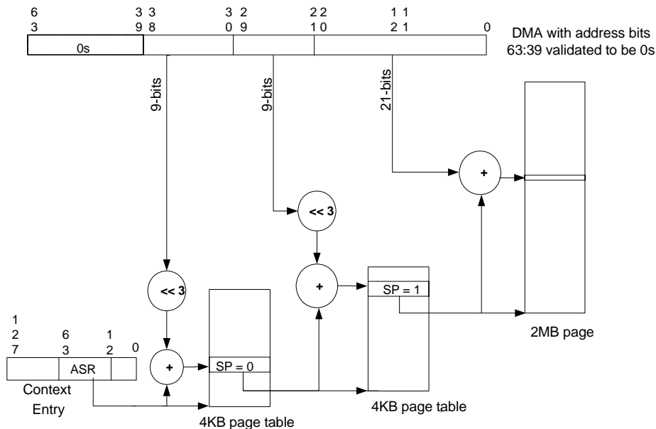
Figure 3-9. Example Multi-level Page Table (with 2MB Super Pages)
