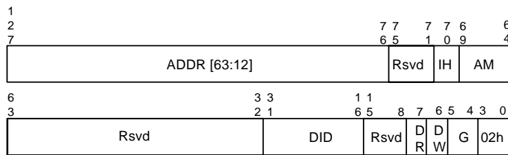
Figure 6-18. IOTLB Invalidate Descriptor
