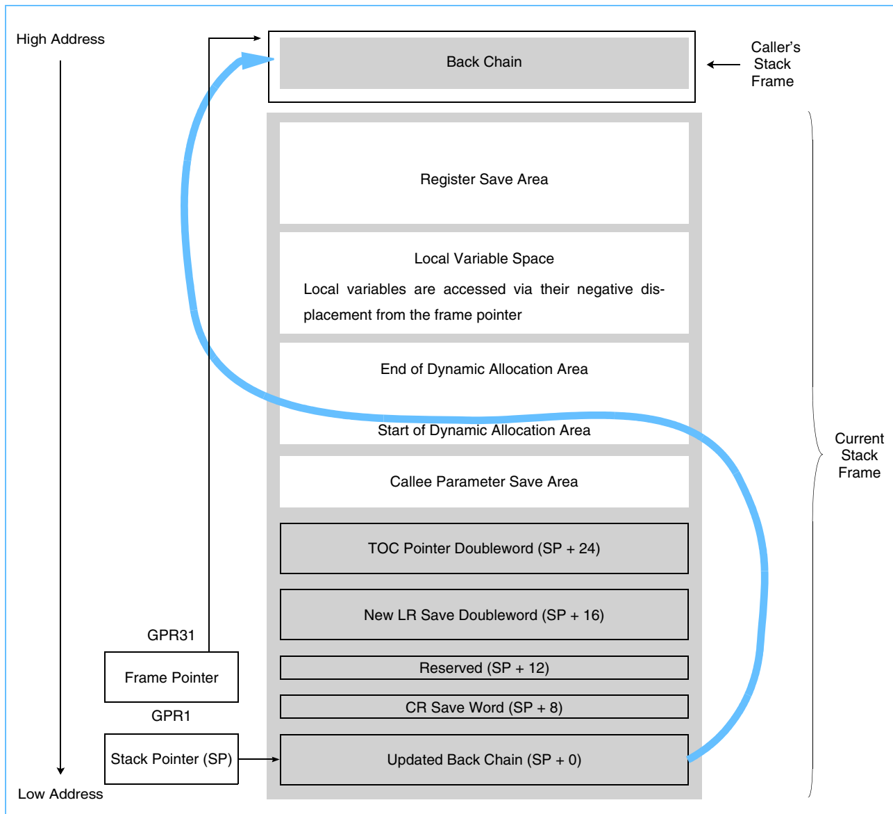
Figure 2-44. After Dynamic Stack Allocation
