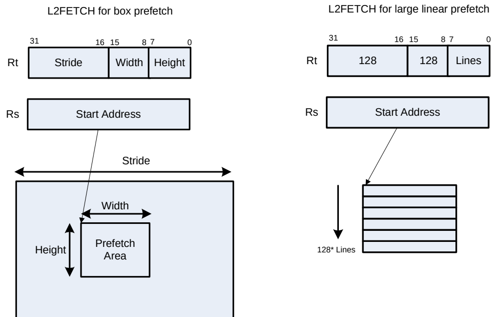
Figure 5-2 L2FETCH instruction
